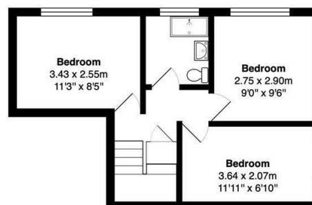
Second Floor Area: 35.3 m 2 ... 380 ft 2
